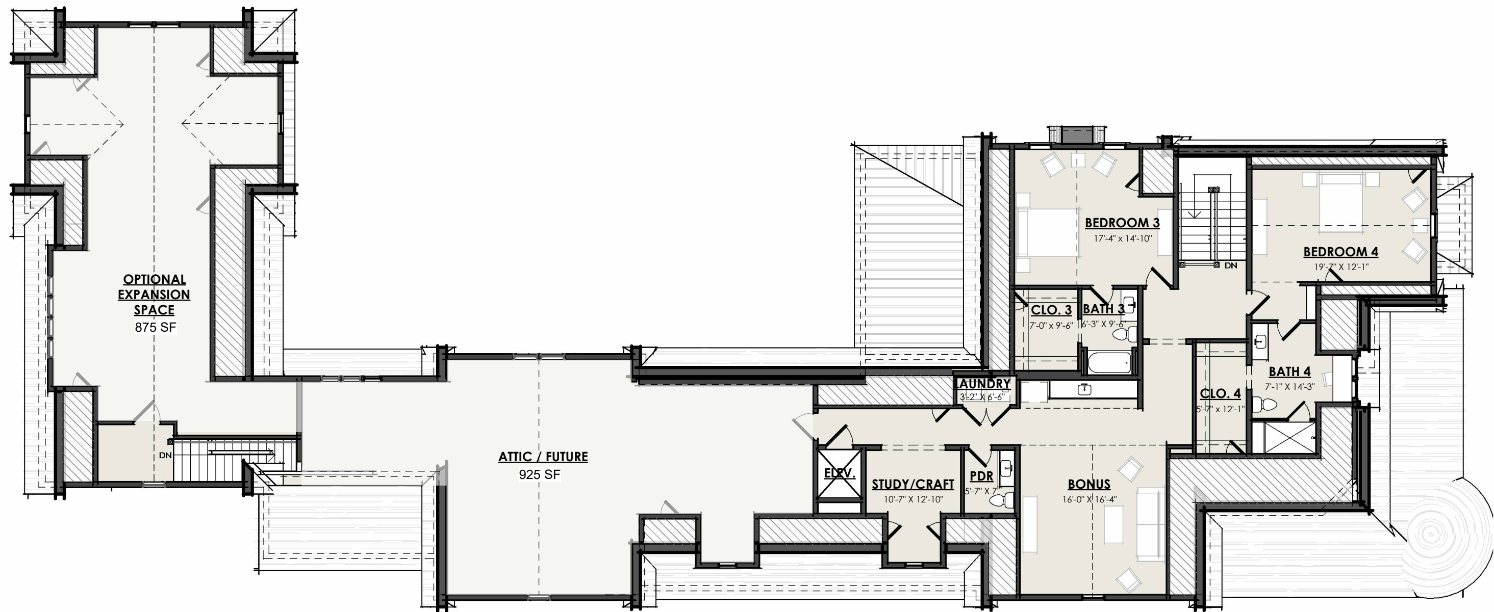
SECOND FLOOR PLAN 3/32" = 1'-0"
